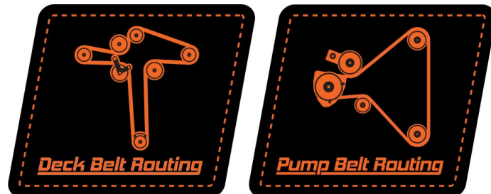
491-0082-00 Deck Belt and Pump Routing Decal
