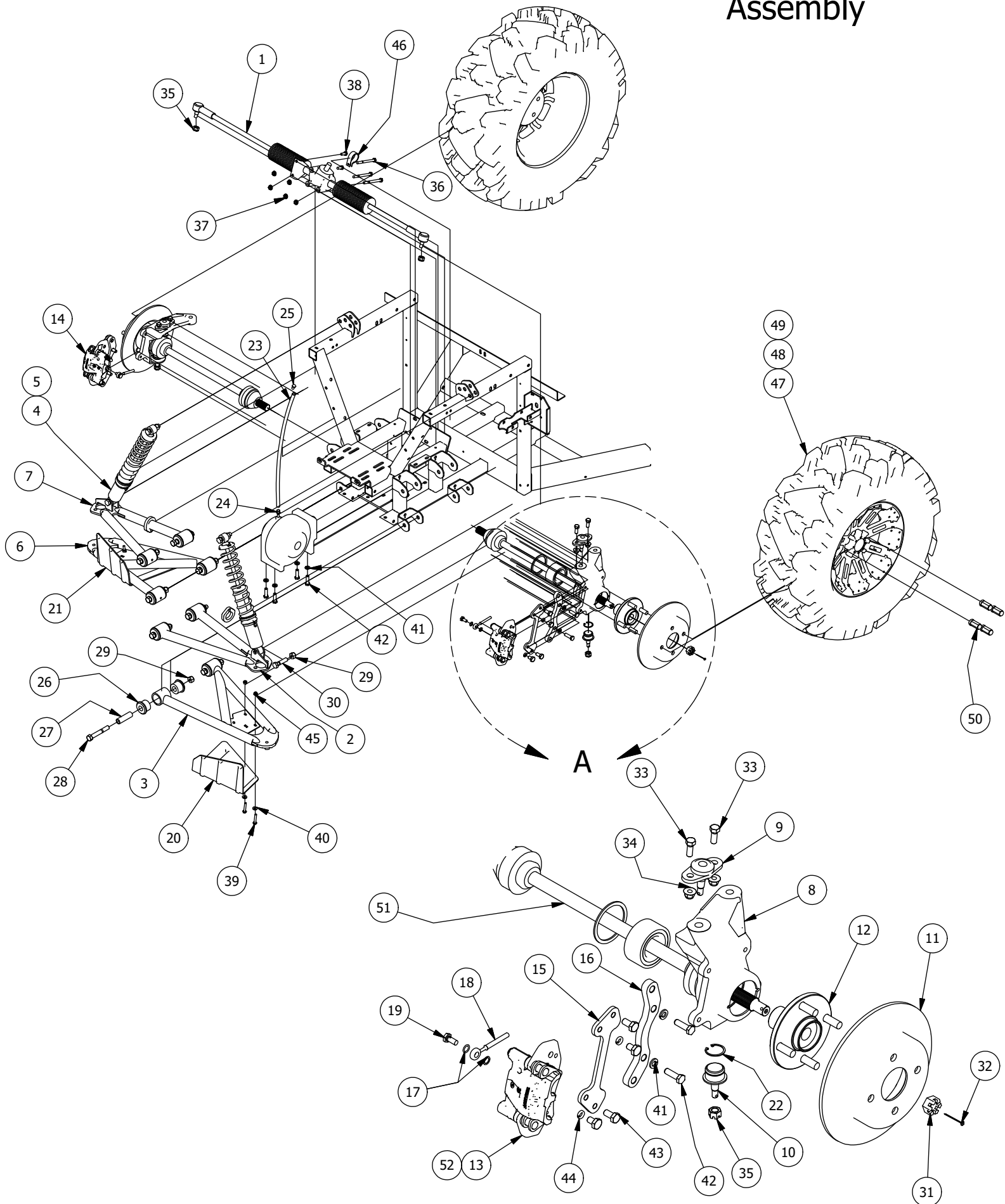
DETAIL A
