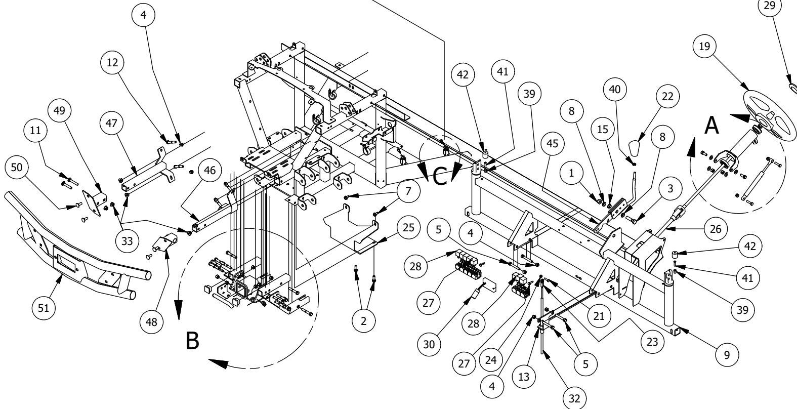
DETAIL A
