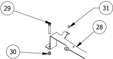
DETAIL B
