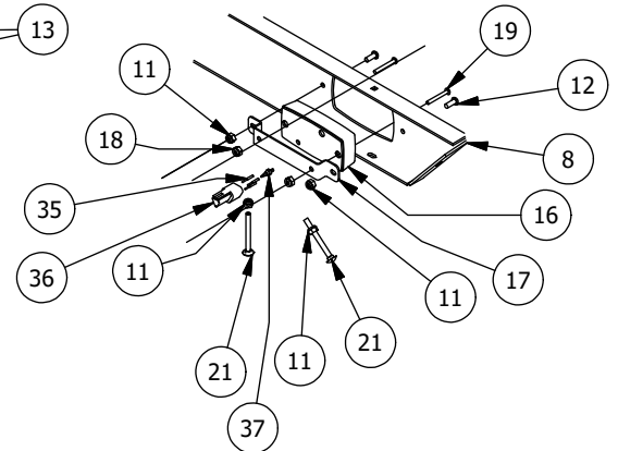
DETAIL C
