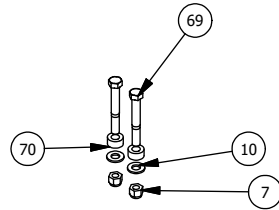
DETAIL D
