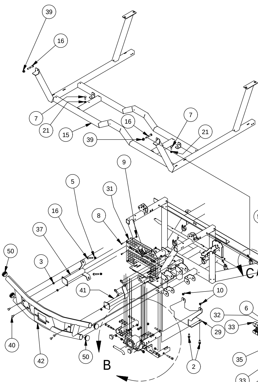
DETAIL A
