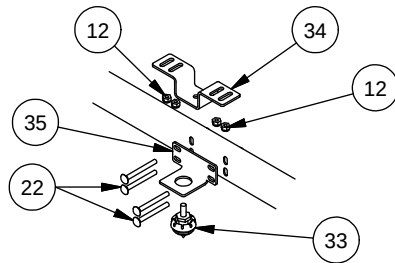
DETAIL E
