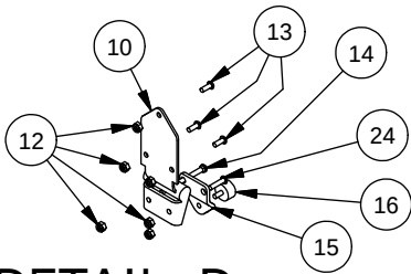
DETAIL D
