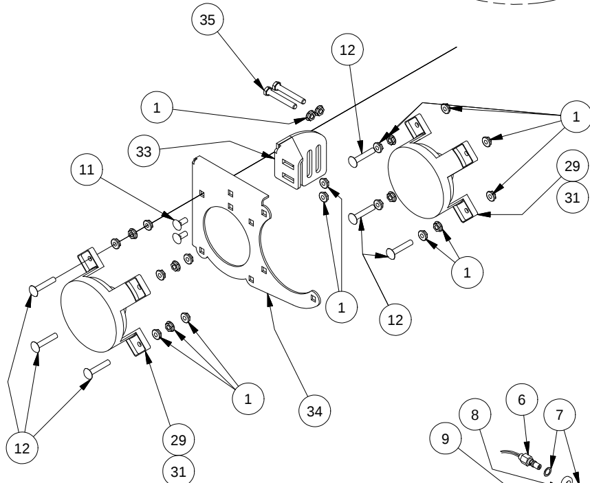
DETAIL B
