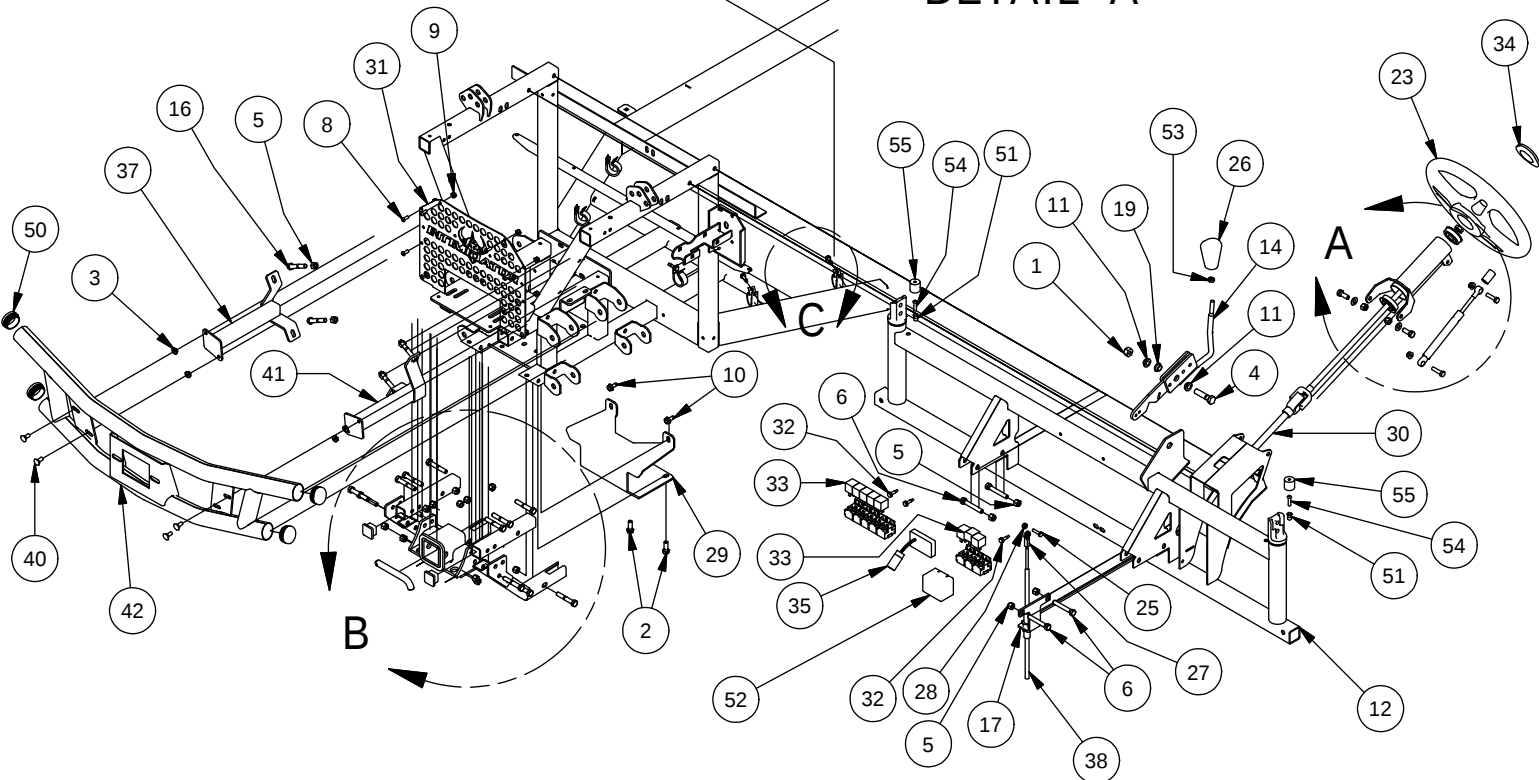
DETAIL A
