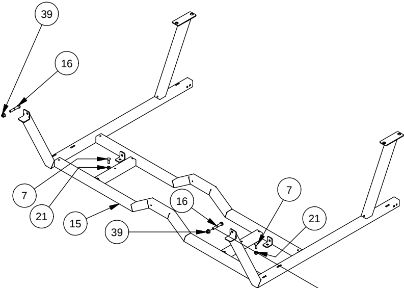
DETAIL B
