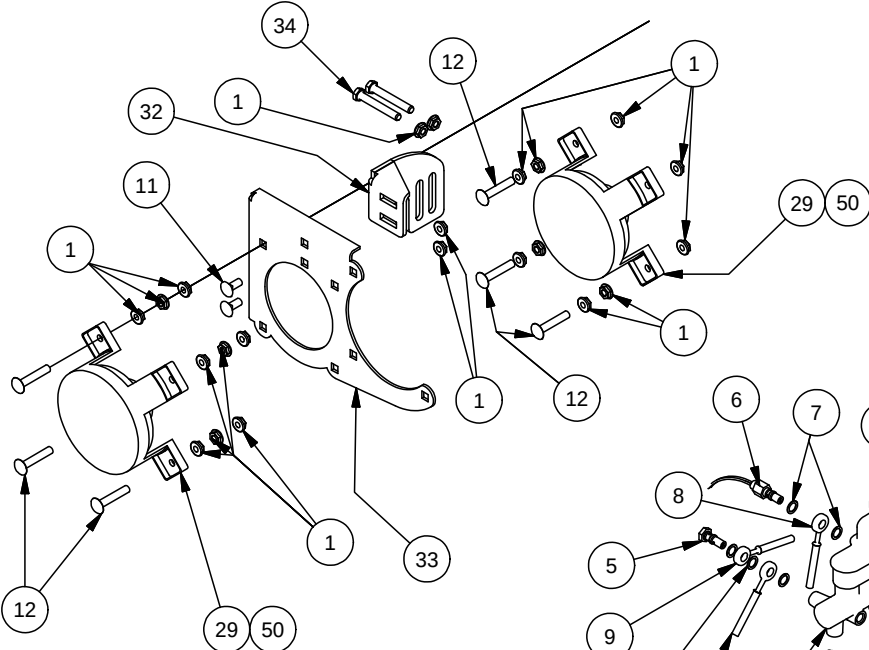
DETAIL B
